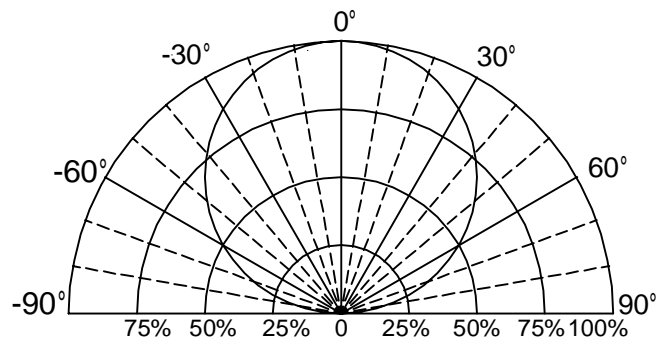
Fig.6 Directive Radiation
