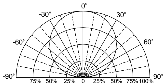
Fig.6 Directive Radiation
